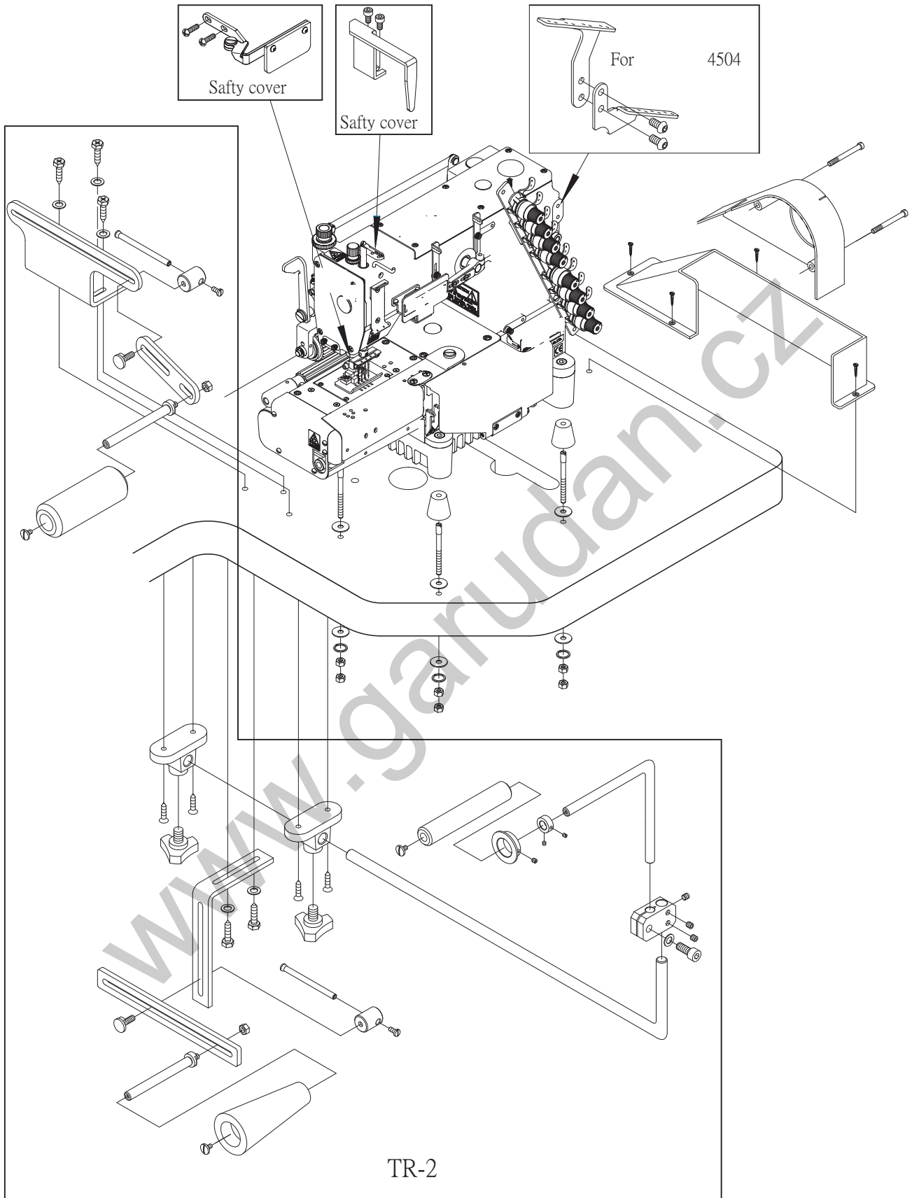
TR-2 Fabric Tension Controlling Device For ( 4504P)
