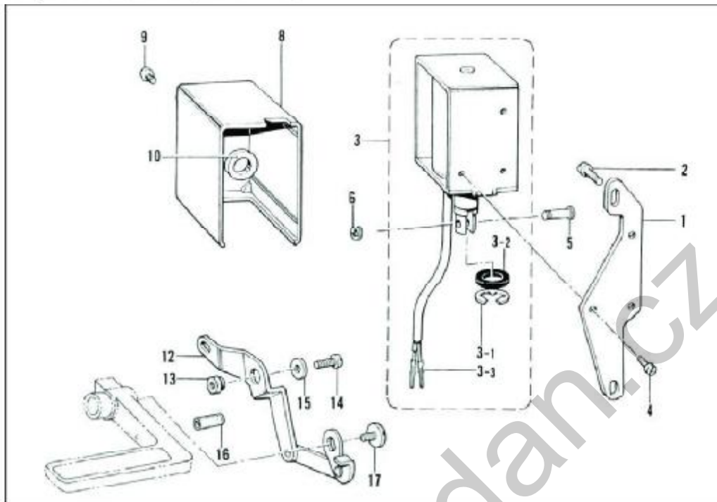
J. Lower shaft mechanism
